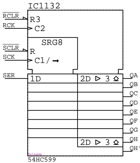
54HC599 IC????
