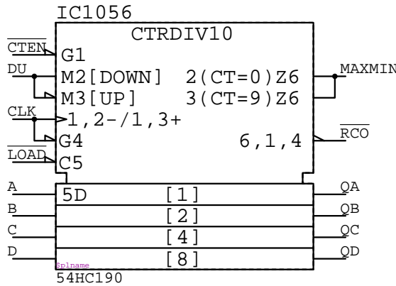
54HC190 IC????
