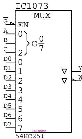
54HC251 IC????
