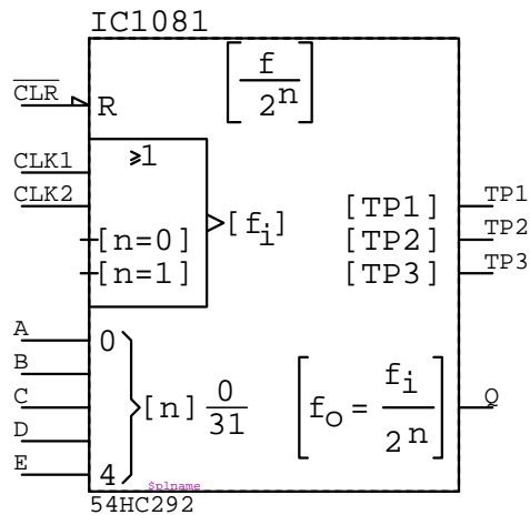
54HC292 IC?????
