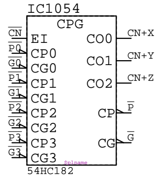
54HC182 IC????
