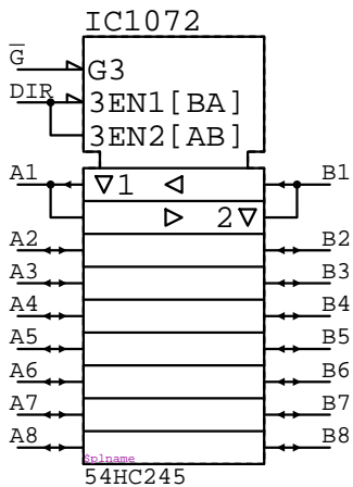
54HC245 IC????
