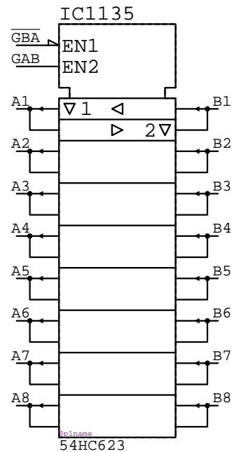
54HC623 IC????
