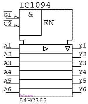
54HC365 IC?????
