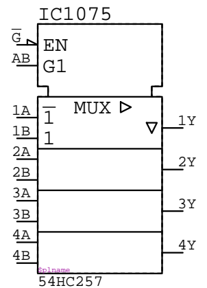
54HC257 IC????
