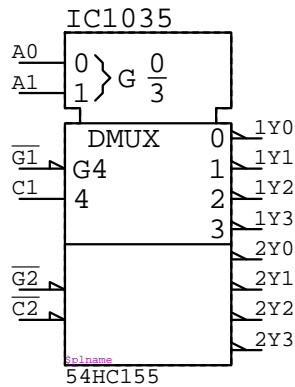
54HC155 IC????
