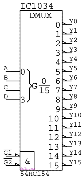
54HC154 IC????
