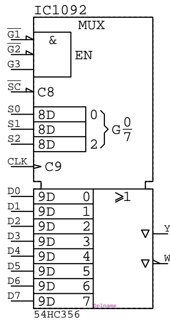
54HC356 IC????
