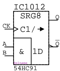
54HC91 IC????
