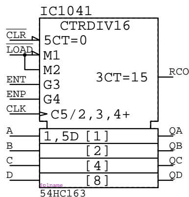
54HC163 IC????
