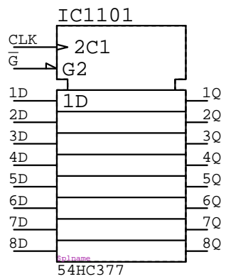
54HC377 IC?????
