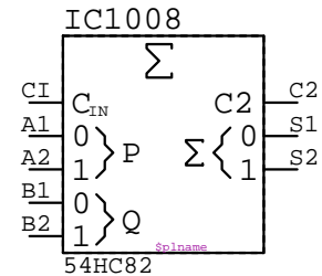
54HC82 IC????
