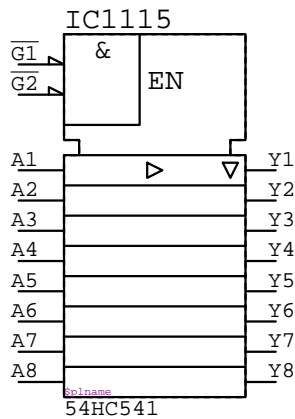
54HC541 IC?????
