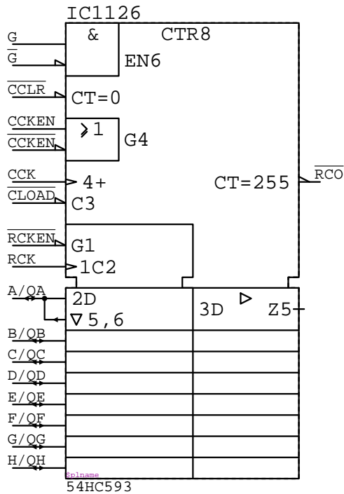
54HC593 IC????
