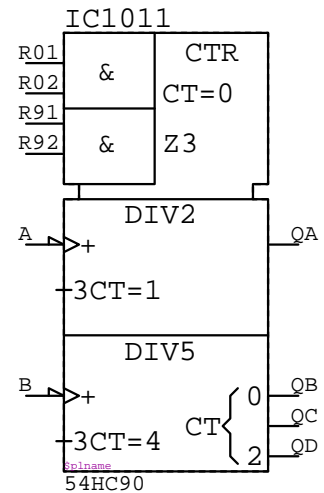
54HC90 IC????
