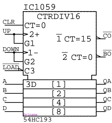
54HC193 IC?????
