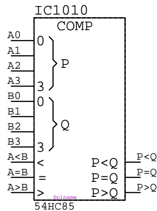
54HC85 IC????
