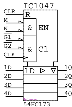
54HC173 IC?????
