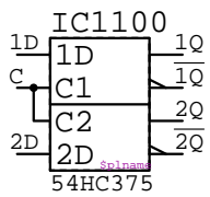
54HC375 IC?????
