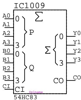
54HC83 IC????
