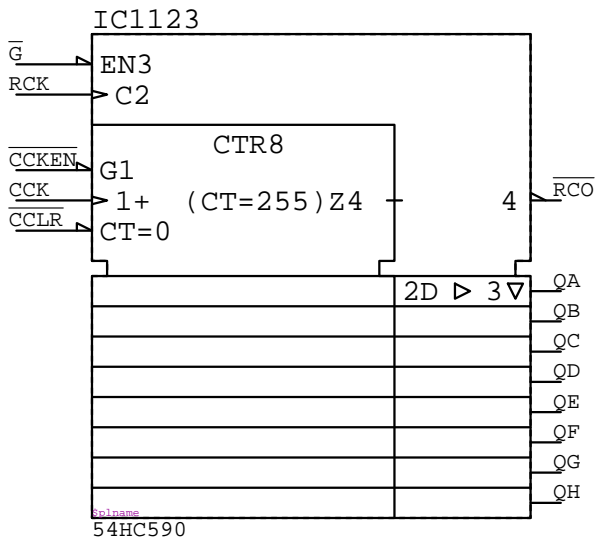
54HC590 IC????
