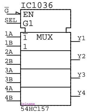
54HC157 IC????
