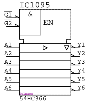
54HC366 IC?????
