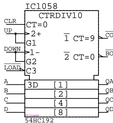
54HC192 IC????
