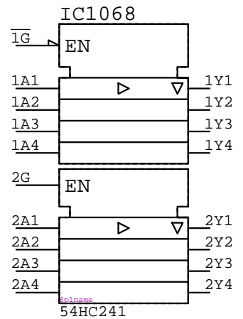
54HC241 IC?????
