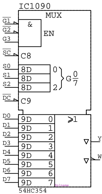
54HC354 IC????
