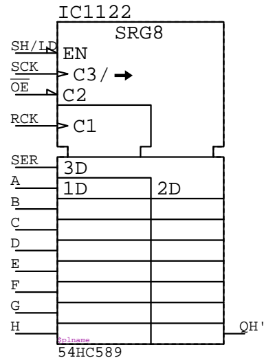
54HC589 IC?????
