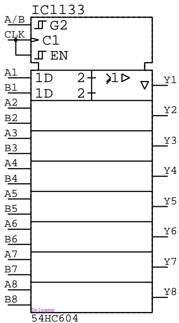
54HC604 IC????
