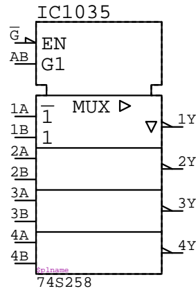
74S258 IC????
