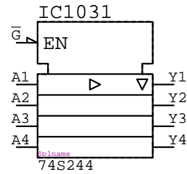
74S244 IC????
