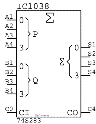
74S283 IC????
