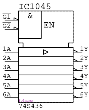
74S436 IC????
