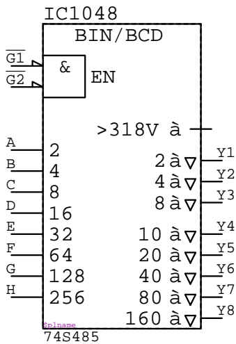
74S485 IC????
