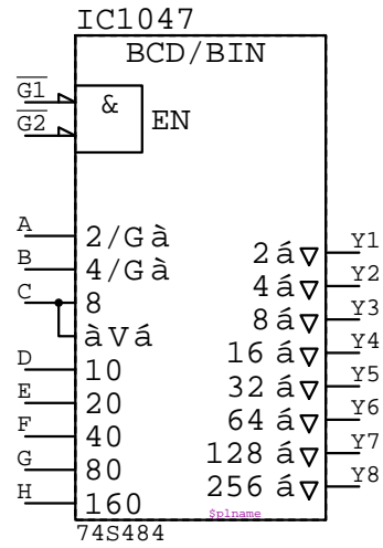
74S484 IC????
