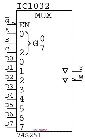
74S251 IC????
