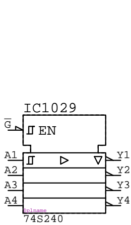
74S240 IC????
