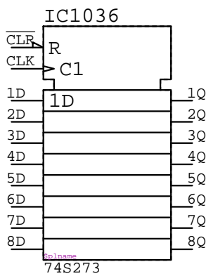
74S273 IC????
