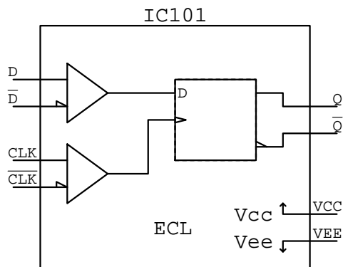
MC100EL52
