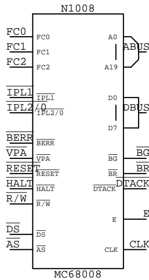
MC68008
