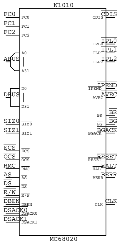
MC68020
