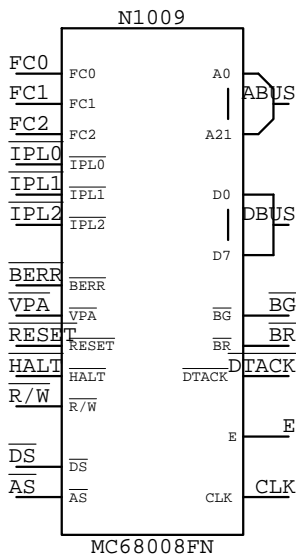
MC68008FN
