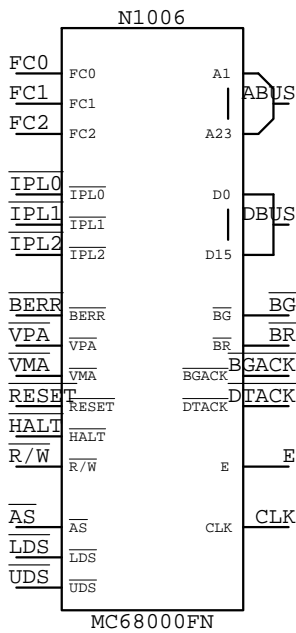
MC68000FN
