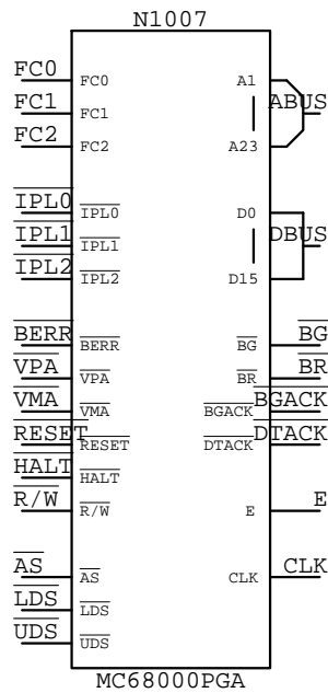
MC68000PGA
